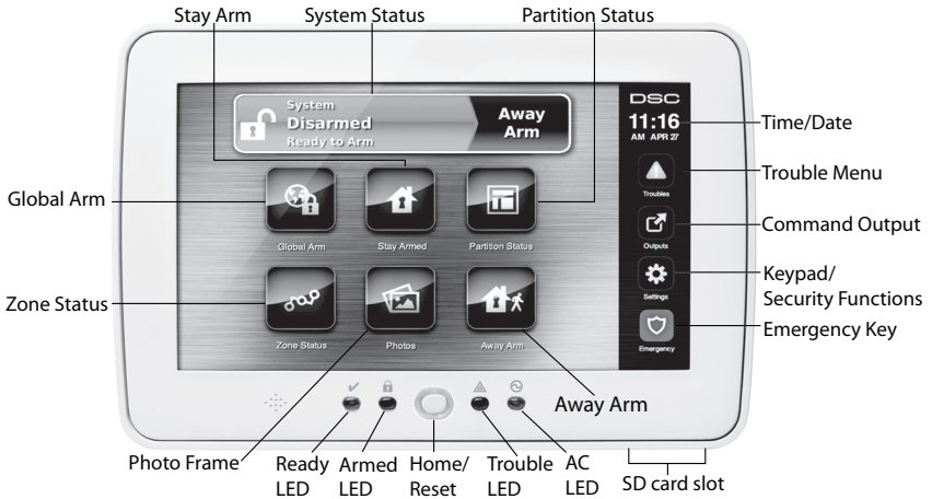
Figure 3 - Controls & Indicators
